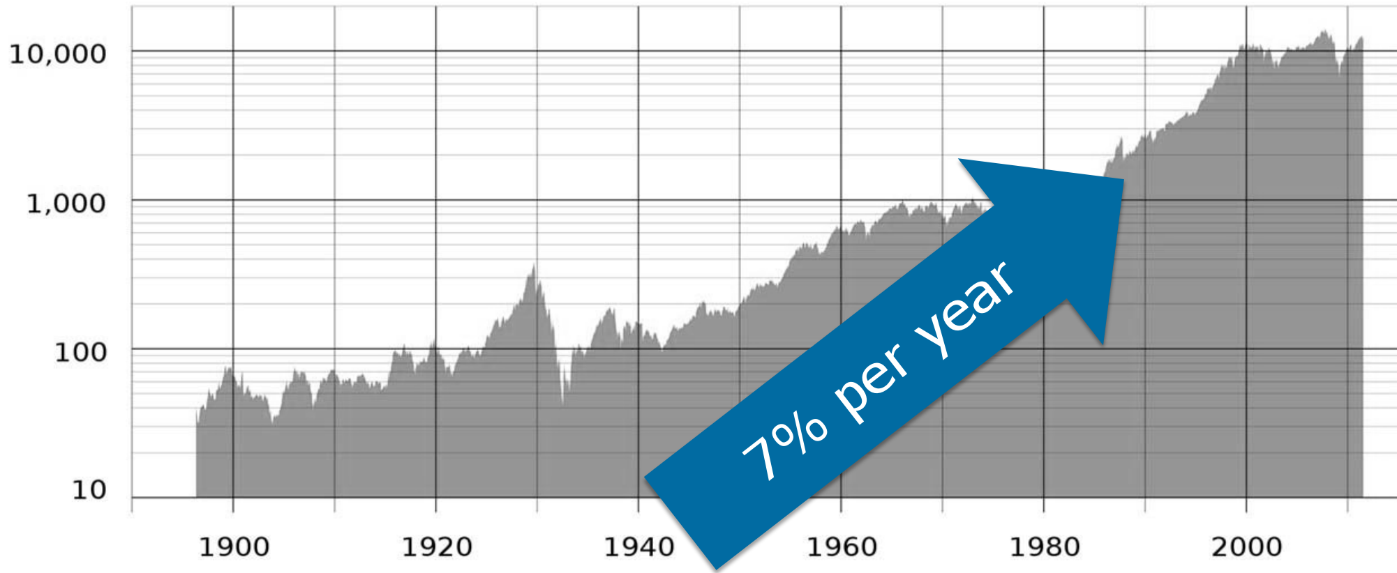
Dow Jones Industrial Average 1896 -2009
